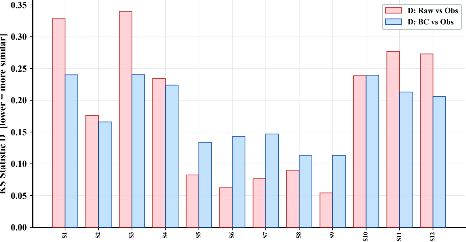
(c) Kolmogorov-Smirnov Test Two-sample: Sim vs Obs (wet days - 1 mm/day)
