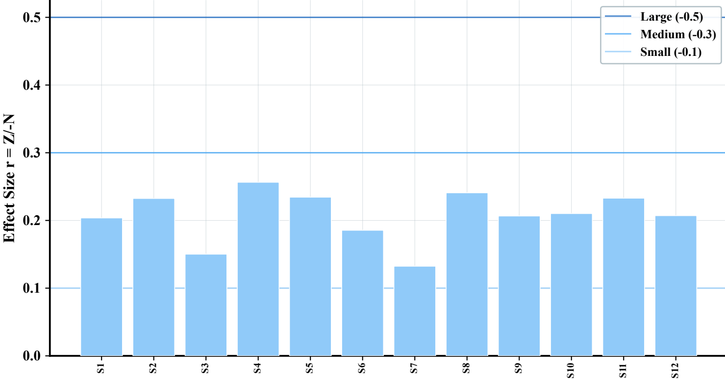
(b) Effect Size (Cohen 1988)
