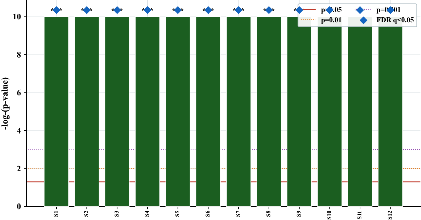
(a) Wilcoxon Signed-Rank Test (one-tailed) H: |err_BC| < |err_Raw|
